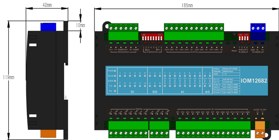
Figure 10: Product dimensions: 185mm * 119mm * 42mm (L × W × H). Weight: 350g
