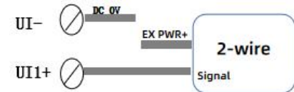
Figure 6: Analog Input Wiring Diagram
