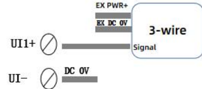
Figure 7: Analog Input Wiring Diagram
